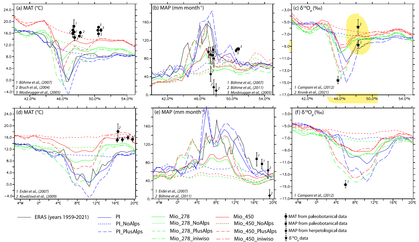
Figure 7. Annual mean temperature (a, d), precipitation (b, e), and \delta^{18}\text{O}_p (c, f) gradients across the Alps: (a–c) averaged between 9°E and 10°E and (d–f) between 46°N and 47°N for topographic sensitivity experiments with pre-industrial (PI_NoAlps, PI, PI_plusAlps) and Middle Miocene (Mio_278, Mio_450, Mio_278_noAlps, Mio_450_noAlps, Mio_278_plusAlps, Mio_450_plusAlps, Mio_278_iniwiso, Mio_450_iniwiso) boundary conditions and for ERA5 reanalysis time averaged from 1959 to 2021. Selected data points (for MAT [Table S1], MAP [Table S1 and Table S2], and \delta^{18}\text{O}_p [Campani et al., 2012; Krsnik et al., 2021]) between 8°E and 11°E (a–c) and between 45°N and 49°N (d–f) extrapolated to the section line are shown in black.
